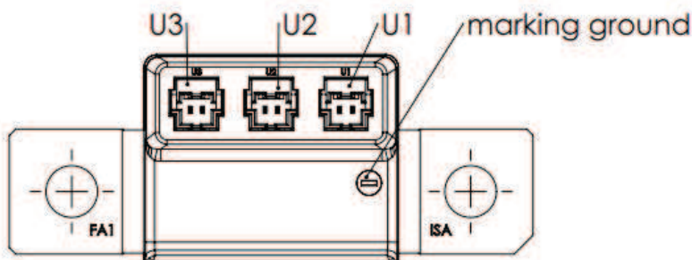
Figure 20: Voltage measurement
