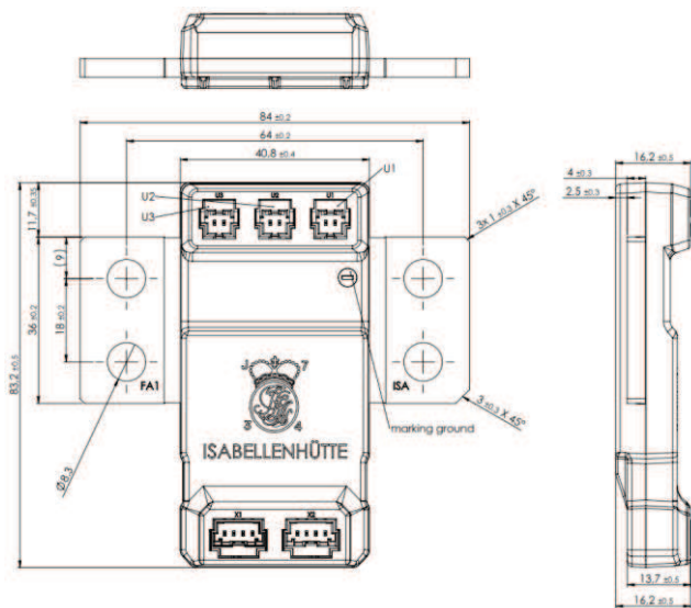
Figure 14: IVT-S 1000A and 2500A version
