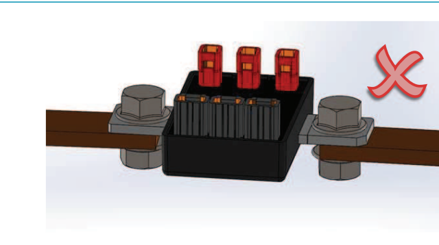
Figure 18: Incorrect mounting 15mm overlap
