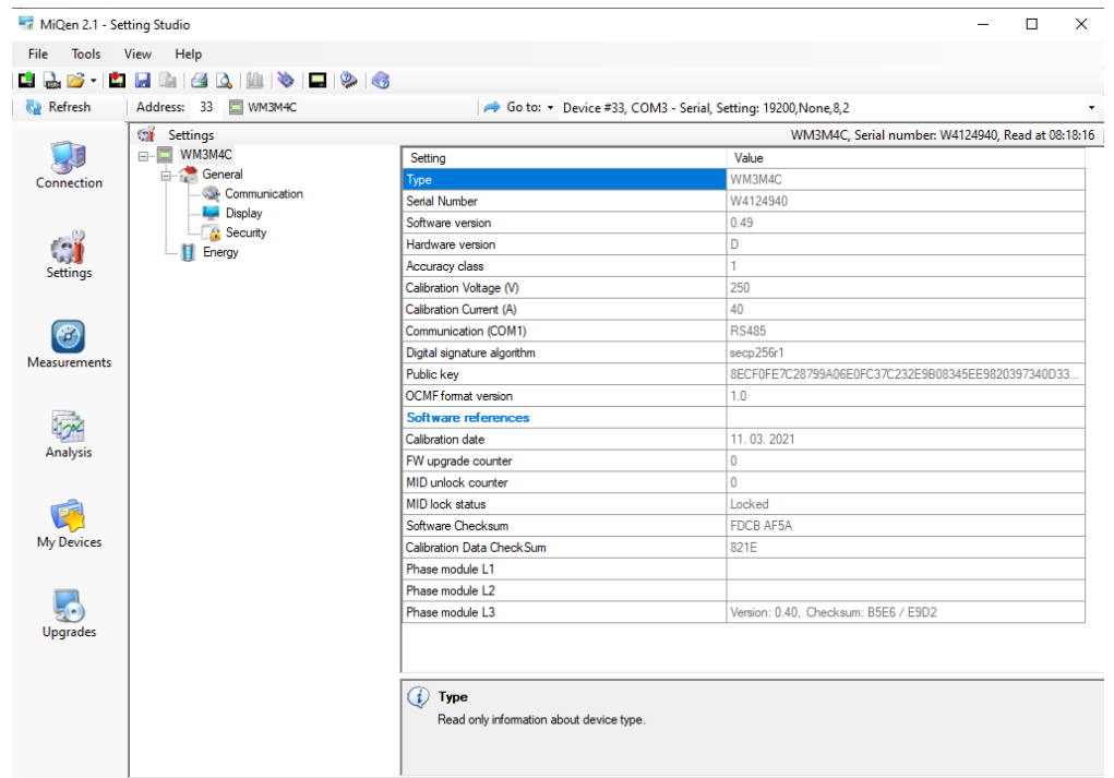
Figure 17: WM3M4C Identification window
