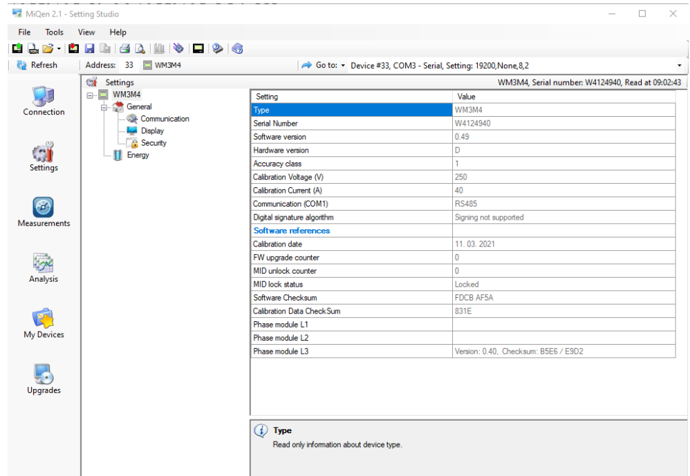
Figure 16: WM3M4 Identification window
