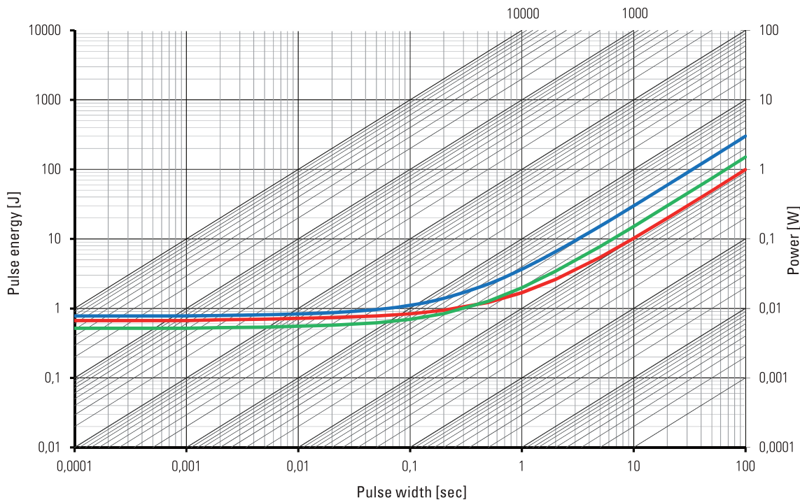
FMS-Z-R0015, FMS-M-R003, FMS-V-R006 Maximum pulse energy / power continuous operation ( T_K = 110\text{ °C} )
