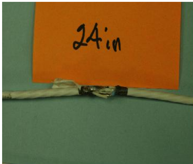
Figure 3: Partial shield fault. The shield remained electrically contiguous with no significant DC resistance. The underlying twisted pair is undamaged.
