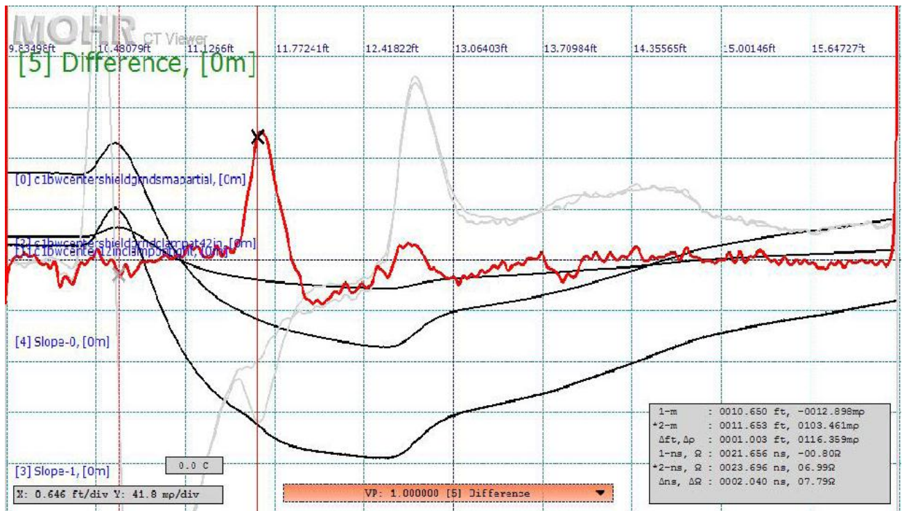
Figure 5: CT Viewer representation of the MIL-STD-1553B databus test setup. The system is tested left to right, with the isolation transformer near the left-hand side of the screen at the location of the dotted (inactive) vertical cursor. The black and gray traces are the raw TDR and 1st derivative traces with the clamp in place and following its removal, with undulation near the left side of the screen representing the inductive effect of the transformer. The fixed gray trace faults near the middle of the screen are due to the fixed partial shield fault. The red trace shows the effect of the shield clamp approximately 1 ft. after the transformer (black X). Notice that the coupling transformer essentially converts the step TDR into a pulse TDR.
