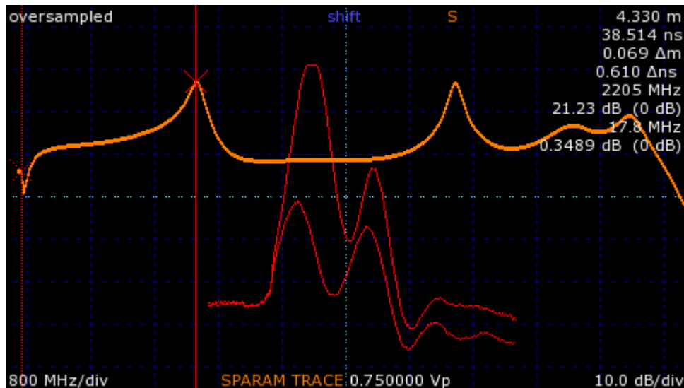
Figure 2: The same 50 Ohm SMA Male-Male coupler as in Fig. 1 now with \sim 7.5 dB excess relative return loss across the first connector. An FFT comparison trace produced from the two faults gives a quick rough estimate of what the dominant reflected frequencies are. Excess return loss at DC is near 0 dB, as expected, with a first peak near 2.2 GHz on the order of 20 dB. Another peak shows up near 5 GHz. However, it is visually obvious from the short wavelength ( \sim 5 cm) of the associated TDR waveform that most of the energy in the 7.5 dB lumped return loss measurement will be centered in the low GHz range, making additional analysis unnecessary.
