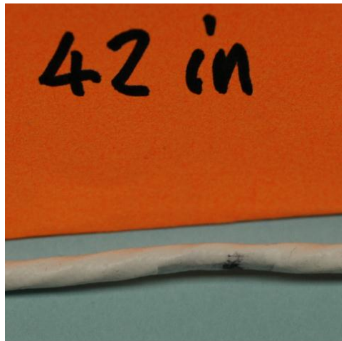
Figure 4: Non-destructive clamp fault, causing deformation of the shield and underlying twisted-pair but no significant permanent damage following its removal. There would likely be no significant impairment of system performance.
